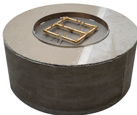
FC42 Circular w/Original Burner
